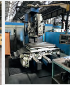
Fraiseuse verticale BOKO type F30 - Courses X 1400 mm - Y 1000 mm - Z 980 mm - Côte SA 50 Table 1400 x 1000 mm Visu 3 axes HEIDENHAIN
